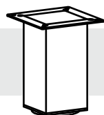
Pata Acero/ Steel Leg H = 80mm
