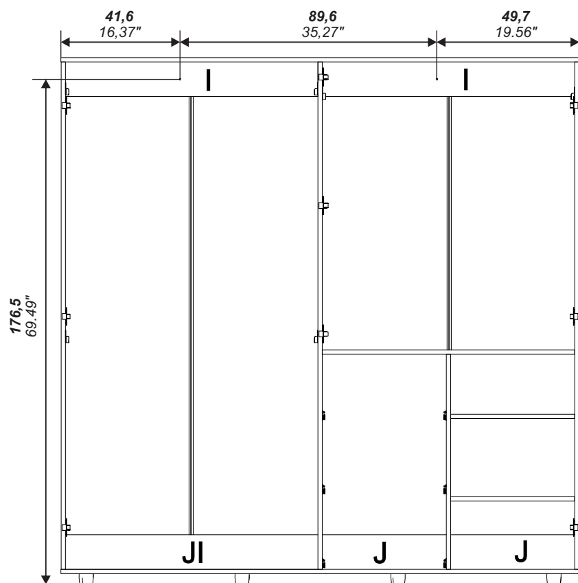
PARED/WALL VISTA FRONTAL / FRONT VIEW
