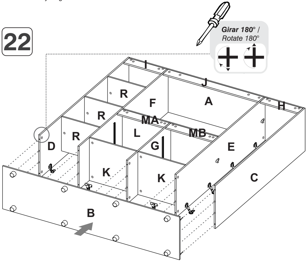
Bisagra parche/ Full overlay hinge
